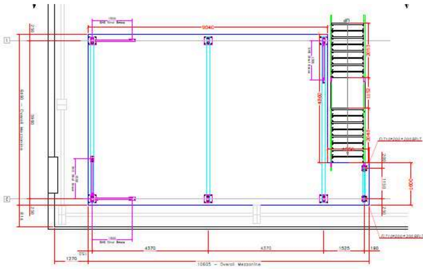
GROUND FLOOR- MEZZANINE STEEL WORK LAYOUT
