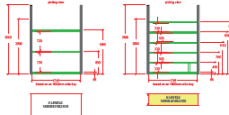
EXAMPLE ELEVATIONS (1:50) SECOND & THIRD LEVELS
